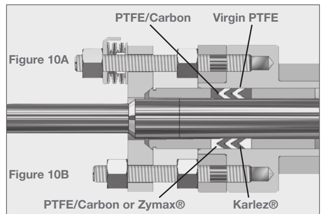
Figure 10A: PT Packing Set
