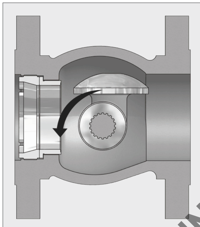
Figure 2: Valve Open
