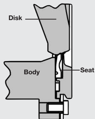
Figure 9: Dual Seat
