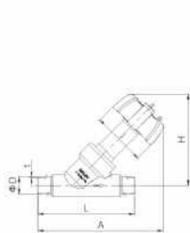
手动角座阀 Manual Angle seat valve NO.VJZ100S1
