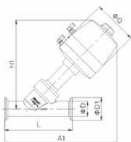
气动角座阀 Pneumatic Angle seat valve NO.VJZ110Q2
