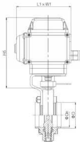
电动蝶阀 Electric actuator butterfly valve NO. VDF100D1
