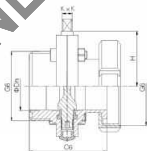
单螺纹单螺母式MALE/NUT(DS) NO.DS-VDF120XX-23
