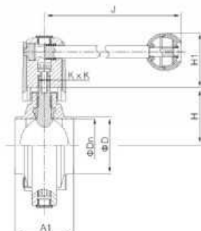
拉式手柄蝶阀 Manual butterfly valve NO. VDF100S1
