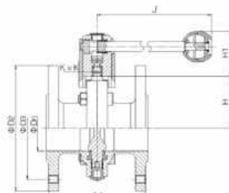
法兰式(圆形) Flange butterfly valve(Round type) NO.VDF240S1
