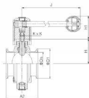
拉式手柄蝶阀 Manual butterfly valve NO.VDF110S1
