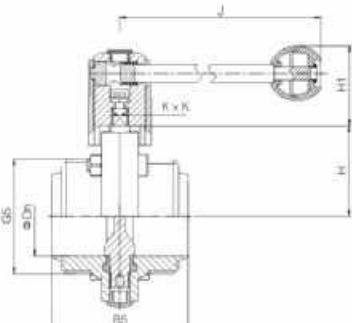
拉手柄蝶阀 Manual butterfly valve with pull handle NO.RJT-VDF130S1
