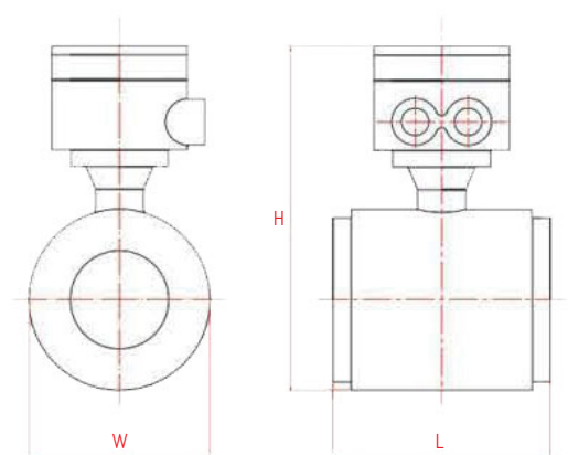
Figuration of clamped type Electromagnetic flow sensor
